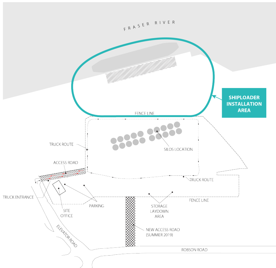
Figure 2: Shiploader Work Area
